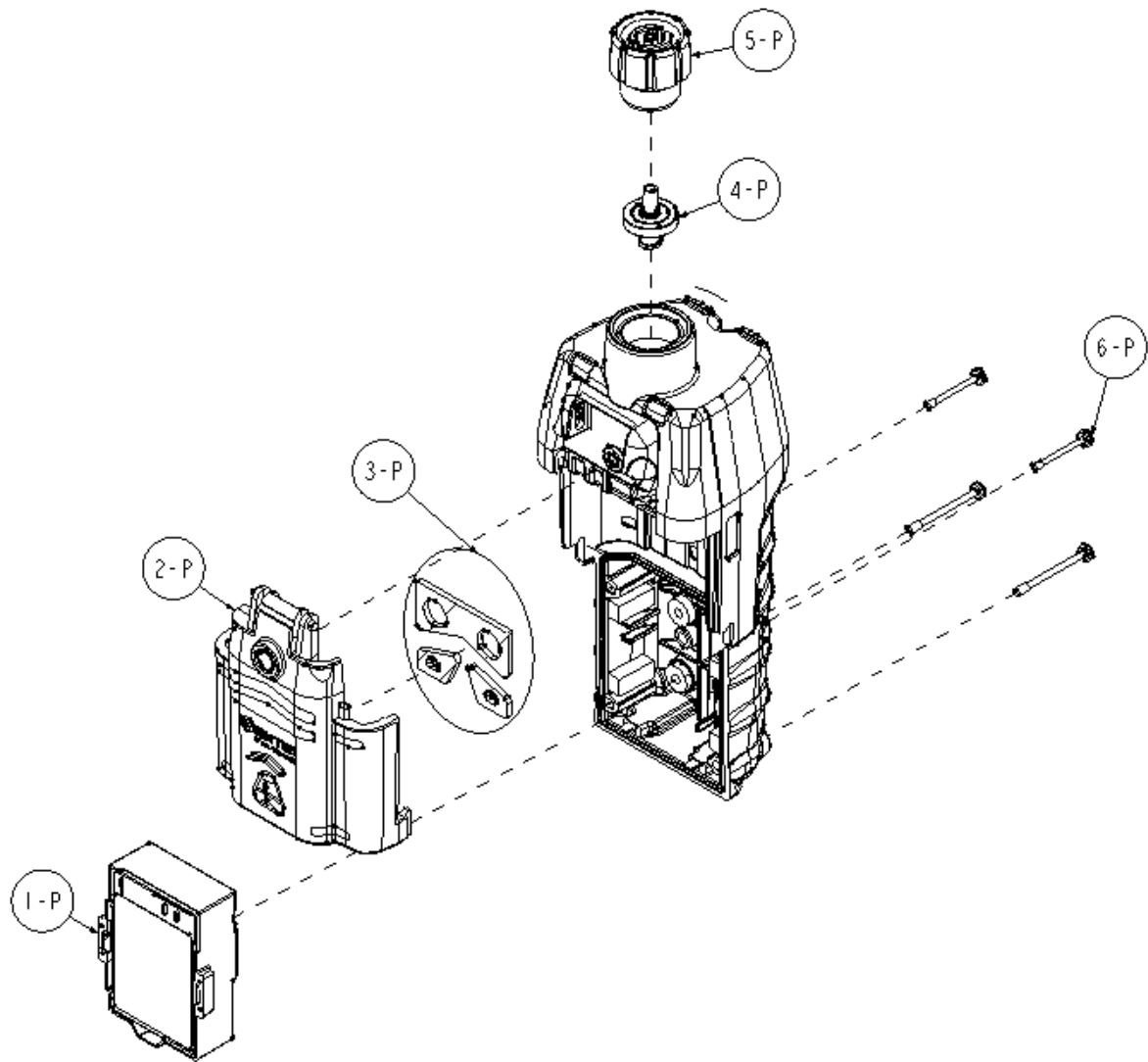
Figure 8.2 Pump module diagram
